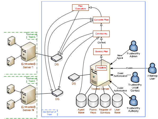
Fig. 2 Distributed architecture designed for management of crisis situations.
